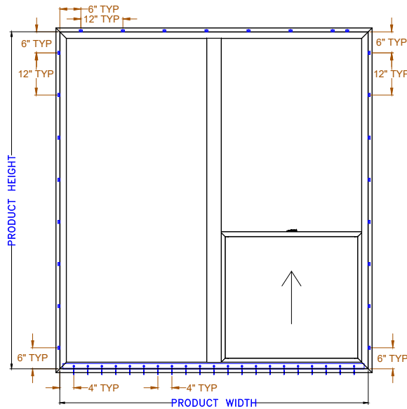
TYPICAL ELEVATION WITH FASTENER SPACING INTERIOR VIEW
