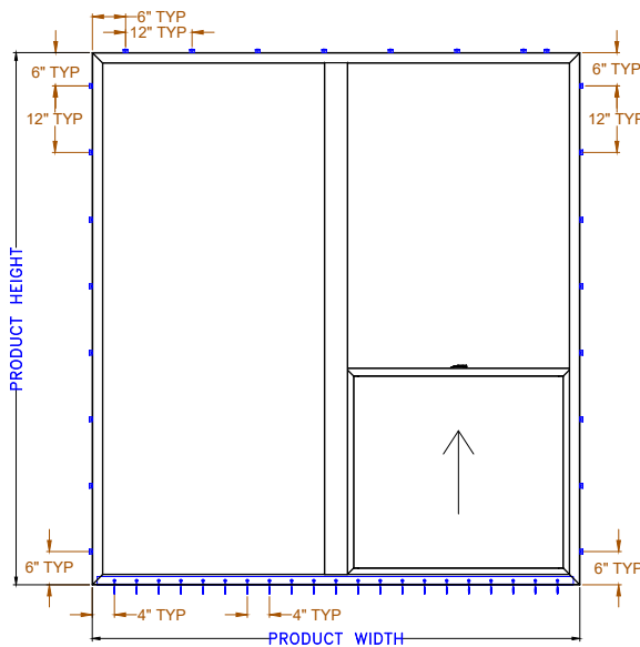
TYPICAL ELEVATION WITH FASTENER SPACING INTERIOR VIEW
