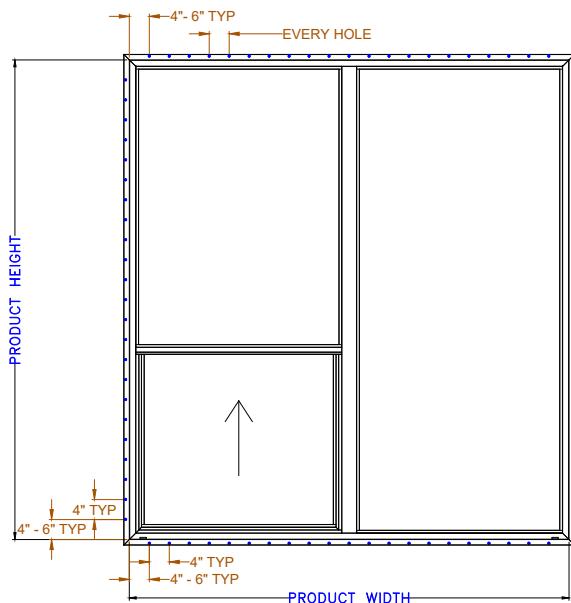
TYPICAL ELEVATION WITH FASTENER SPACING EXTERIOR VIEW
